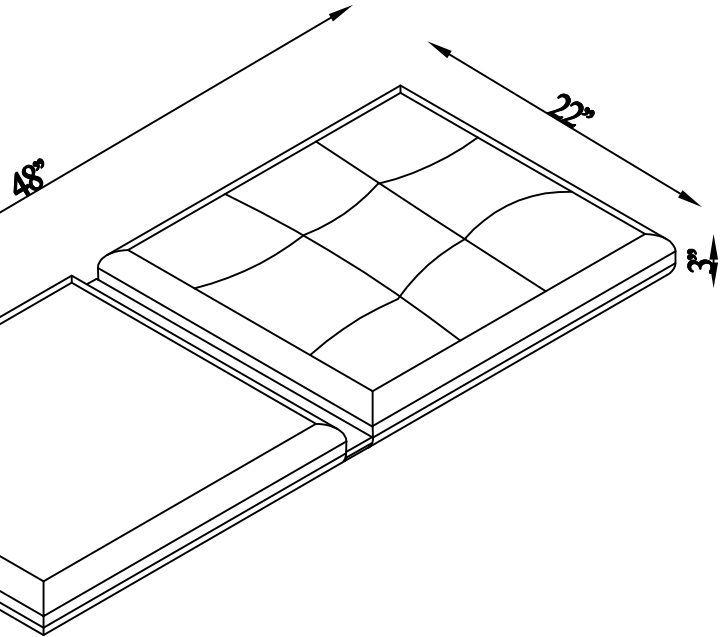
CUSHION
