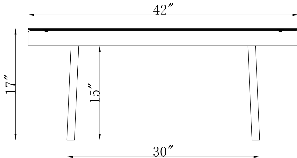
FRONT VIEW
