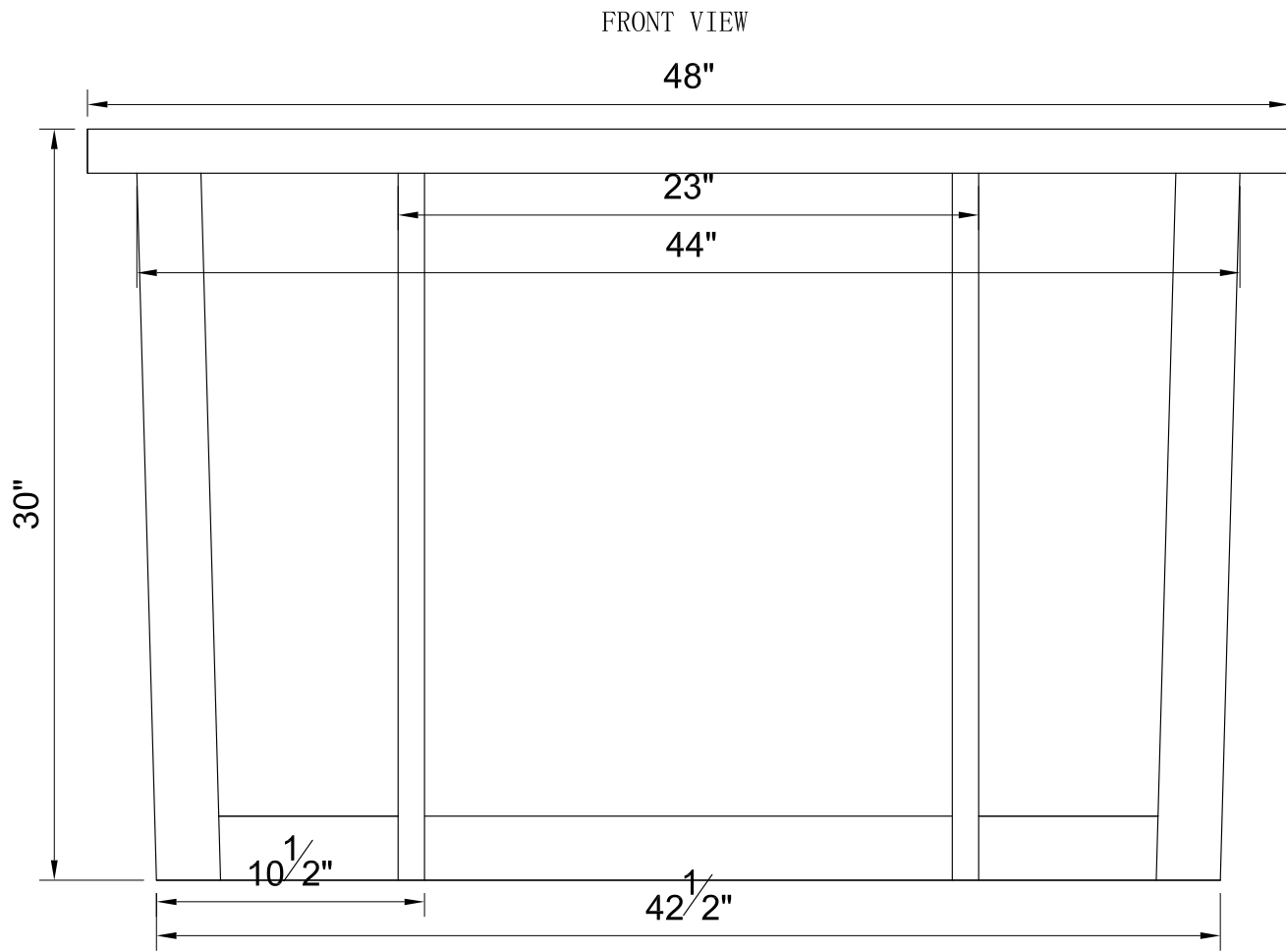
AWBB1020 CONSOLE
