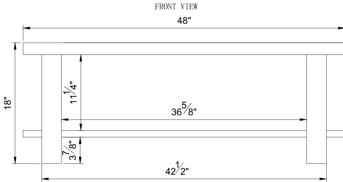
AWAA1220 LARGE COFFEE TABLE
