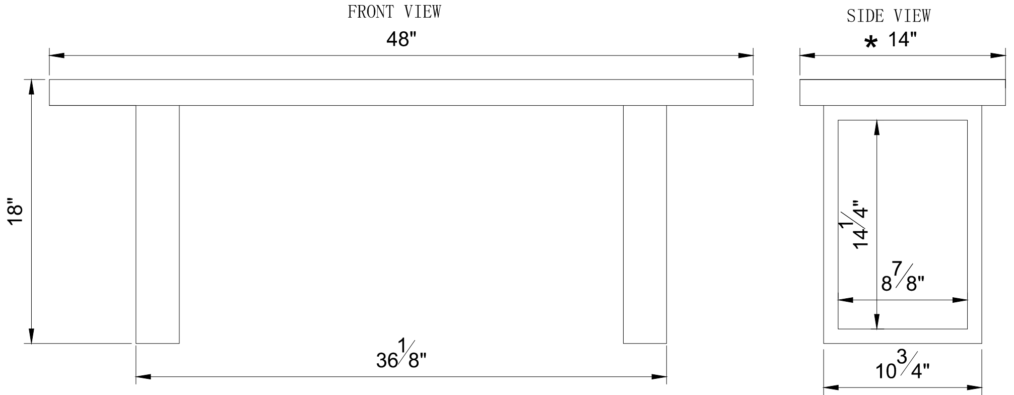
AWAA0420 BENCH 48"
