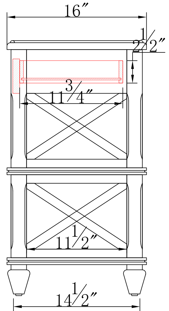
ANSB1062 TV CONSOLE W/DRAWERS
