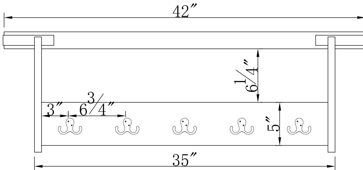
FRONT VIEW
