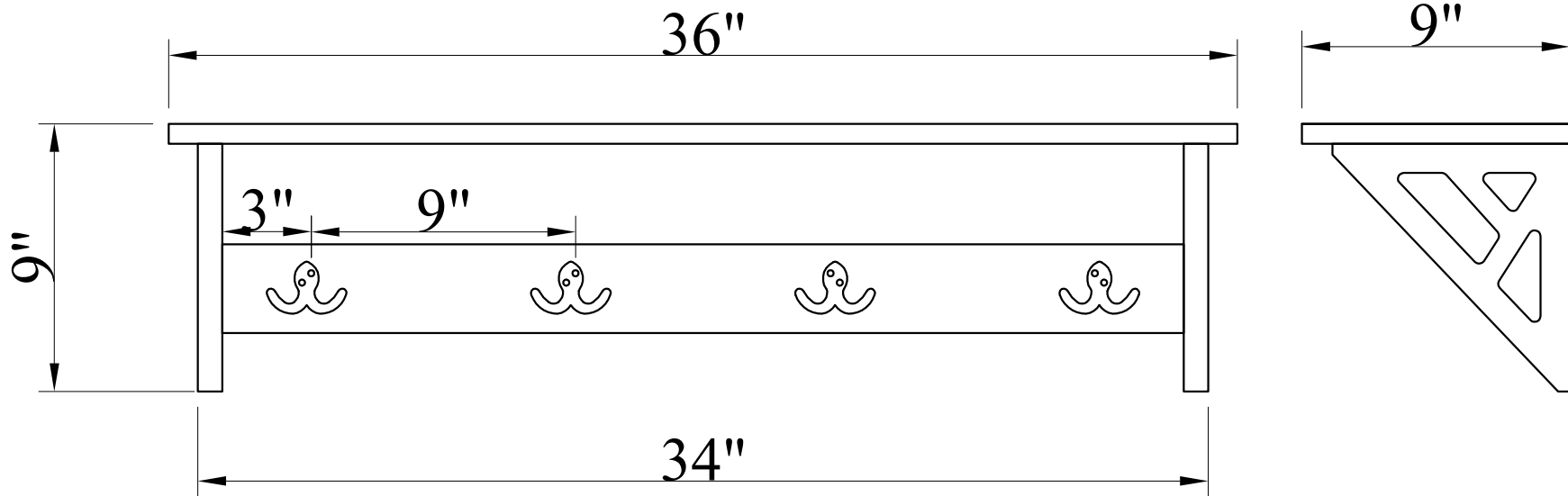
FRONT VIEW
