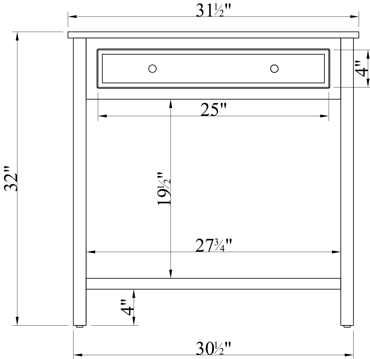
ANCT18 - CONSOLE TABLE WITH 1 DRAWER AND 1 SHELF
