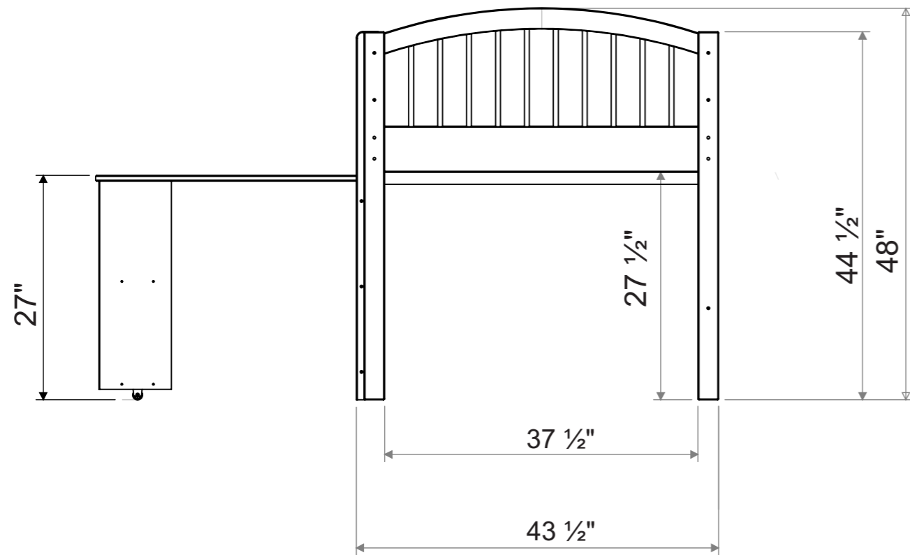
Side View
