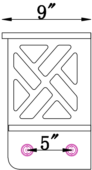
ANCT70WH BATH SHELF WITH 2 TOWEL RODS
