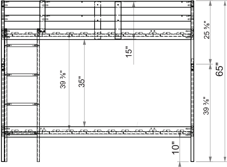
Frontal View
