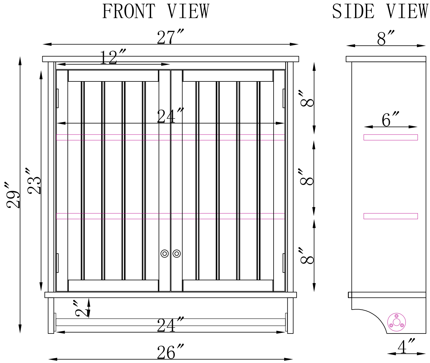
AND073WH 27"W x 29"H WALL MOUNTED BATHROOM STORAGE CABINET WITH 2 DOORS AND TOWEL ROD
