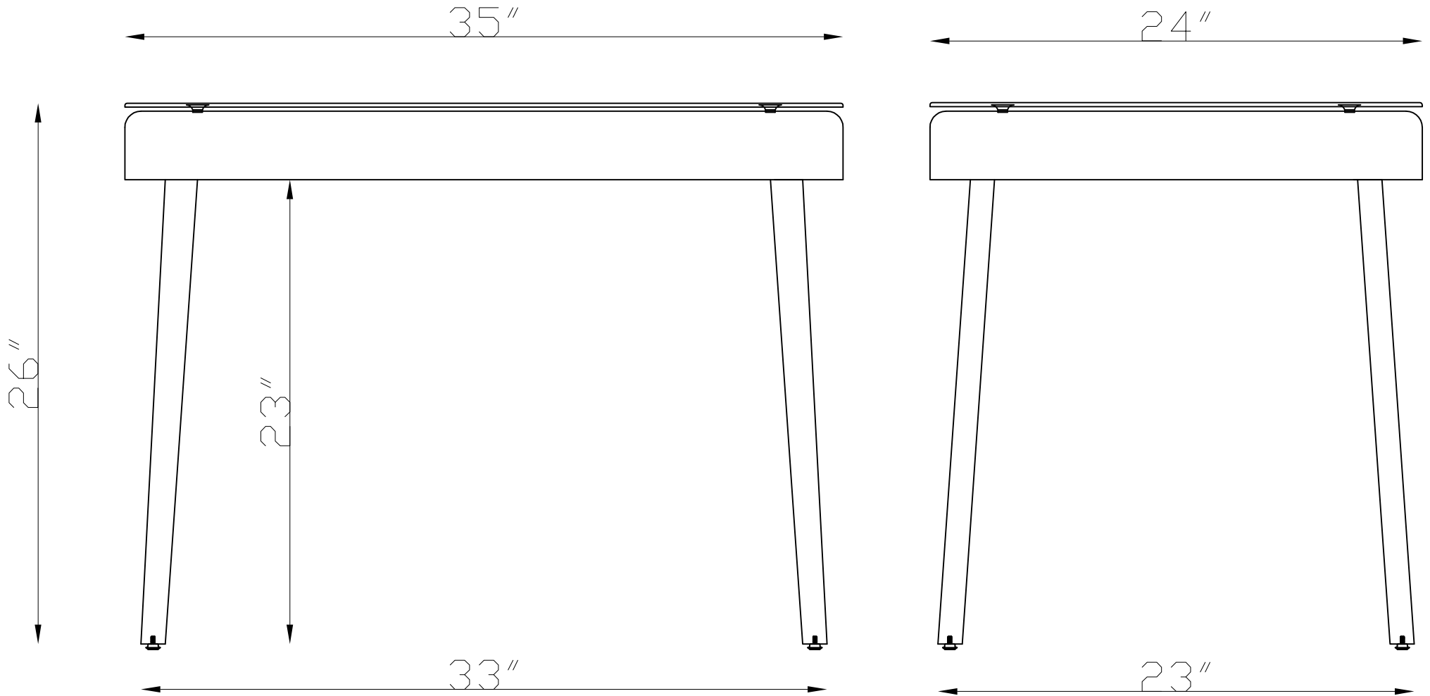
AWWBO4BB-TALL COCKTAIL TABLE
